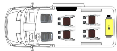
SWB Rear Lift 2 Passenger + 4 WC
