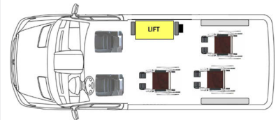
SWB Side Lift 2 Passenger + 3 WC
