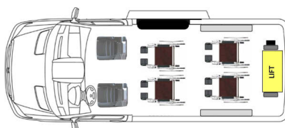
SWB Rear Lift 2 Passenger + 4 WC
