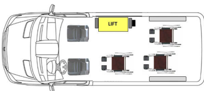
SWB Side Lift 2 Passenger + 3 WC
