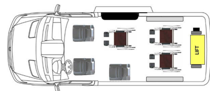
SWB Rear Lift 3 Passenger + 3 WC
