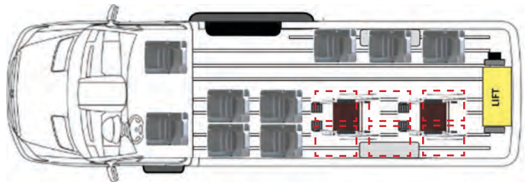
Smartliner seating layout with two wheelchair positions. Six removable seats (outlined in red) can be used in place of wheelchairs for seating up to 15.
